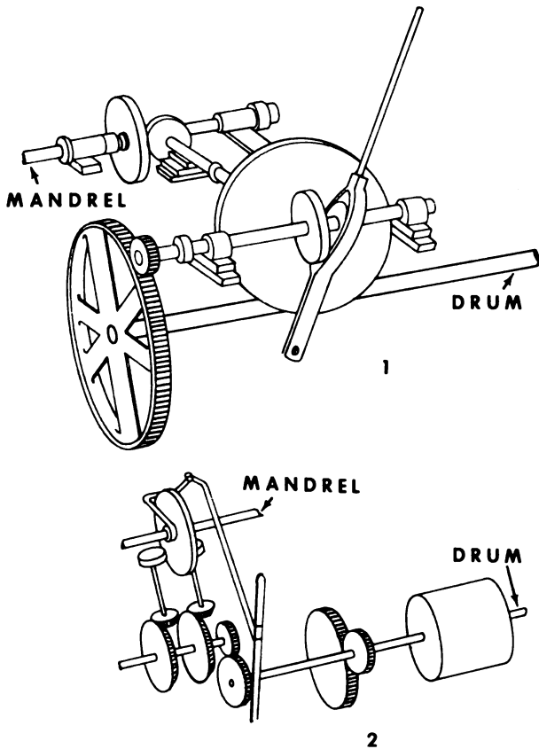
Figure 8-4. Straight friction types of feed works.
